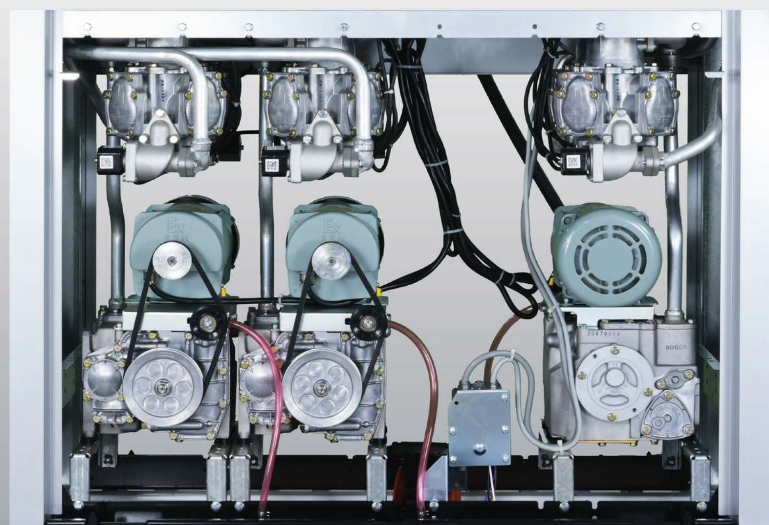
Suction Type
